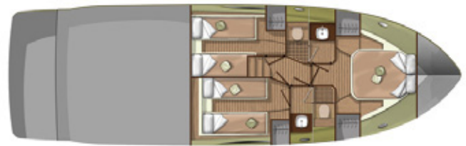
LOWER DECK - 3 CABINS
